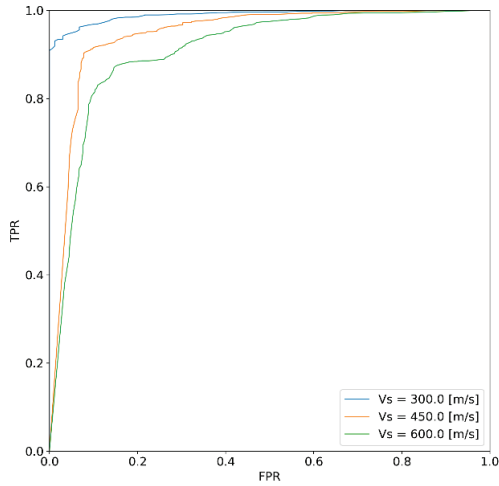
Figure 4 - ROC curves for optimized simple indicator kriging settings.
