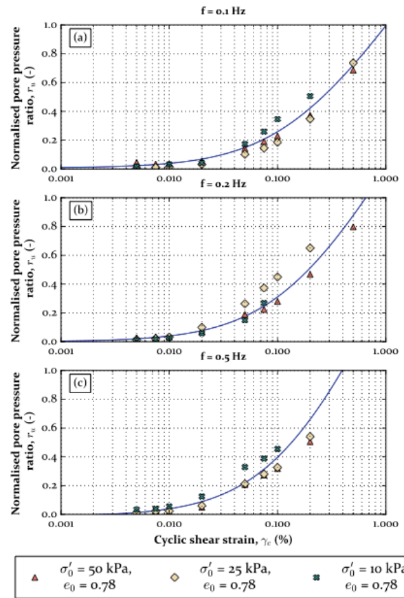
Figure 5 Analytical model for pore pressure build-up [6]: (a) Frequency of 0.1 Hz, (b) Frequency of 0.2 Hz and (c) Frequency of 0.5 Hz.
