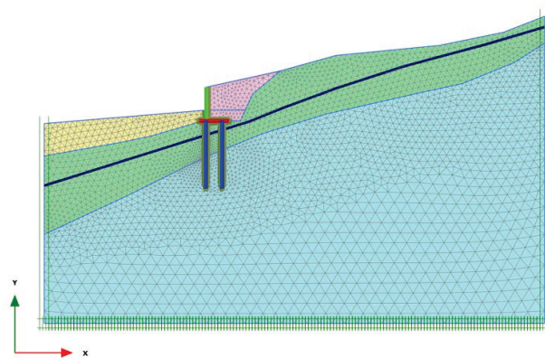
Figure 5 Numerical model used for geotechnical analysis of zone I (reinforced concrete wall with piles) for landslide Laz 18, performed in Bentley Plaxis 2D software.
