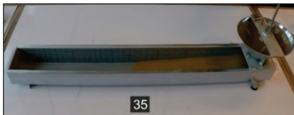
Figure 6 Flow channel.
