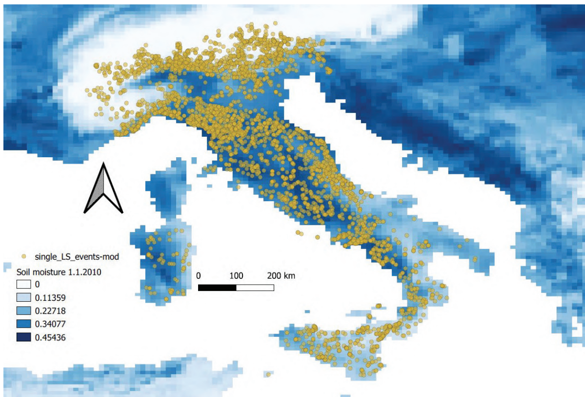
Figure 2 Soil moisture reanalysis data ( m^3/m^3 ) on a specific date (i.e. 1.1.2010) and all the landslides included in the FranelItalia database. Adopted after Bezak et al. (2021).
